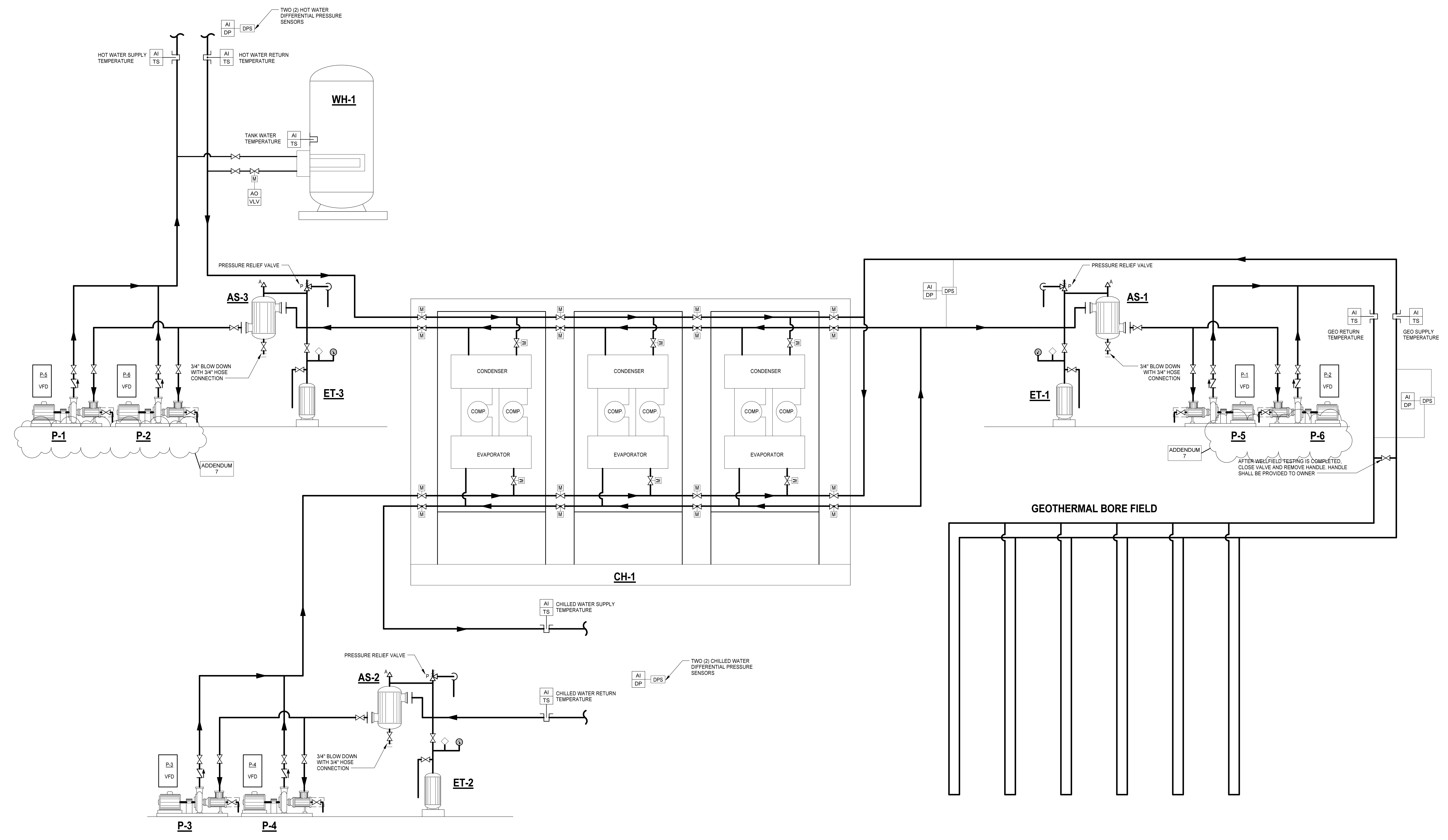
HYDRONIC WATER SYSTEM SCHEMATIC NO SCALE
