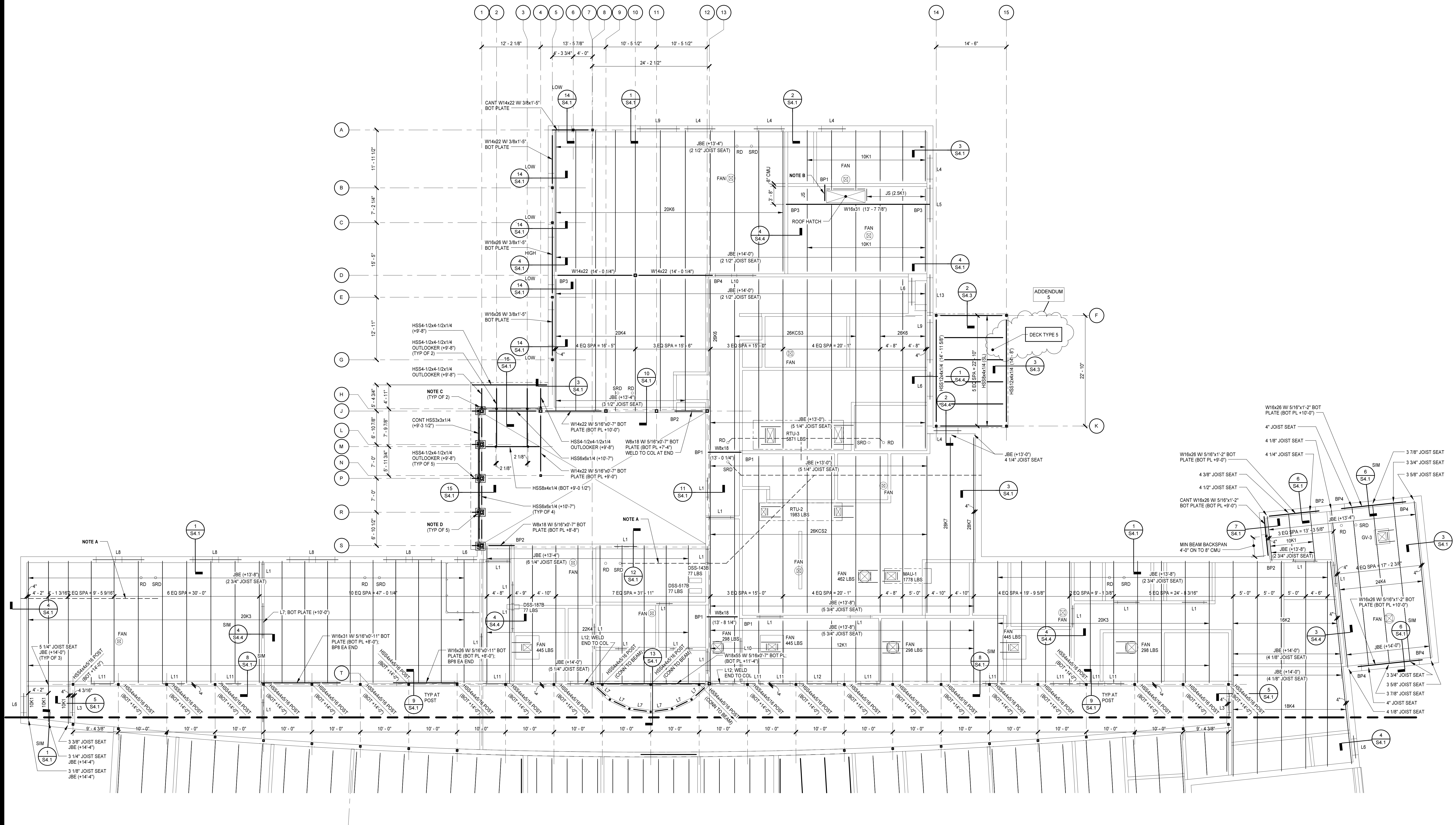
LOW ROOF FRAMING PLAN - PART A 1/8" = 1'-0"
