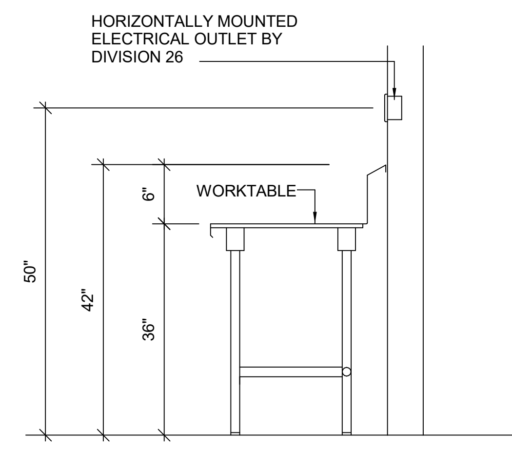
TYPICAL UNASSIGNED WALL OUTLET DETAIL NO SCALE
