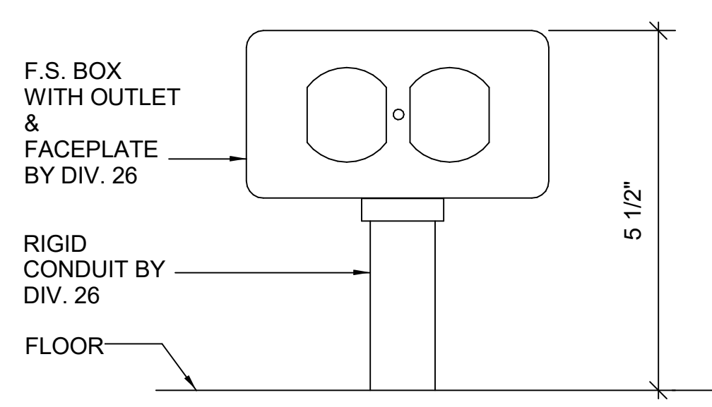
FLOOR RECEPTACLE NO SCALE
